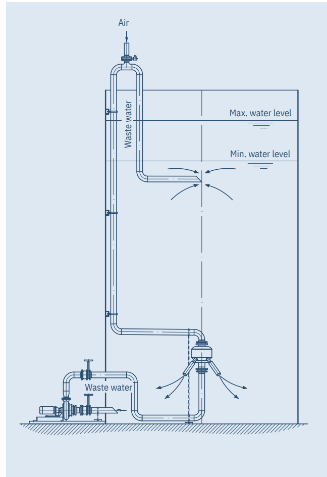
SBR with atmospheric air intake
